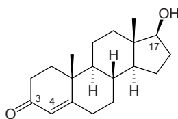
Testosteron (17β-Hydroxy-4-androsten-3-on)
