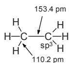
Ethan
