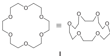
I [18]Krone-6 (18K6) 1,4,7,10,13,16-Hexaoxacyloctadecan
