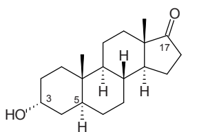
Androsteron (5α-Androstan-3α-ol-17-on)
