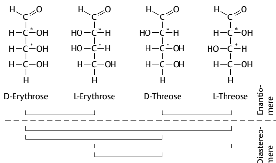
Abb. 3.41 Stereoisomere von 2,3,4-Trihydroxybutanal
