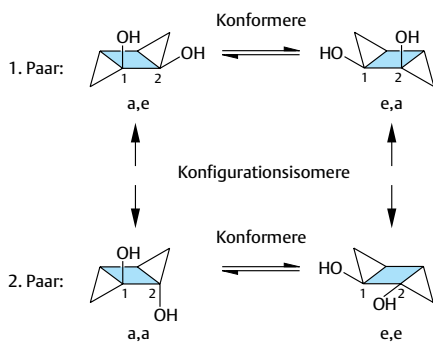
Abb. 3.30 Konformations- und Konfigurationsisomere des Cyclohexan-1,2-diols (a = axial, e = equatorial)
