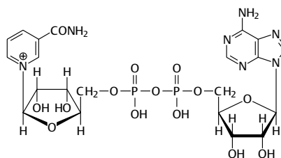
Abb. 3.20 Nicotinamid-adenin-dinucleotid (NAD + )
