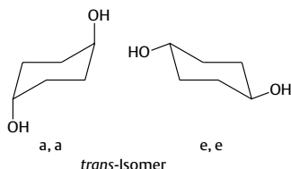
Cyclohexan-1,4-diol
