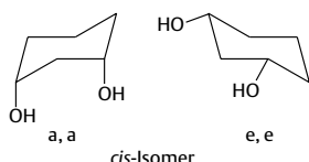
Cyclohexan-1,3-diol
