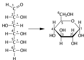
D-Glucose
