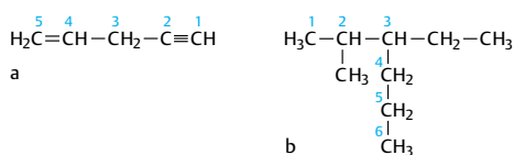
Abb. 3.14 (a) Pent-4-en-1-in, (b) 3-Ethyl-2-methyl-hexan
