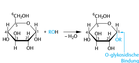
\alpha -D-Glucopyranose
