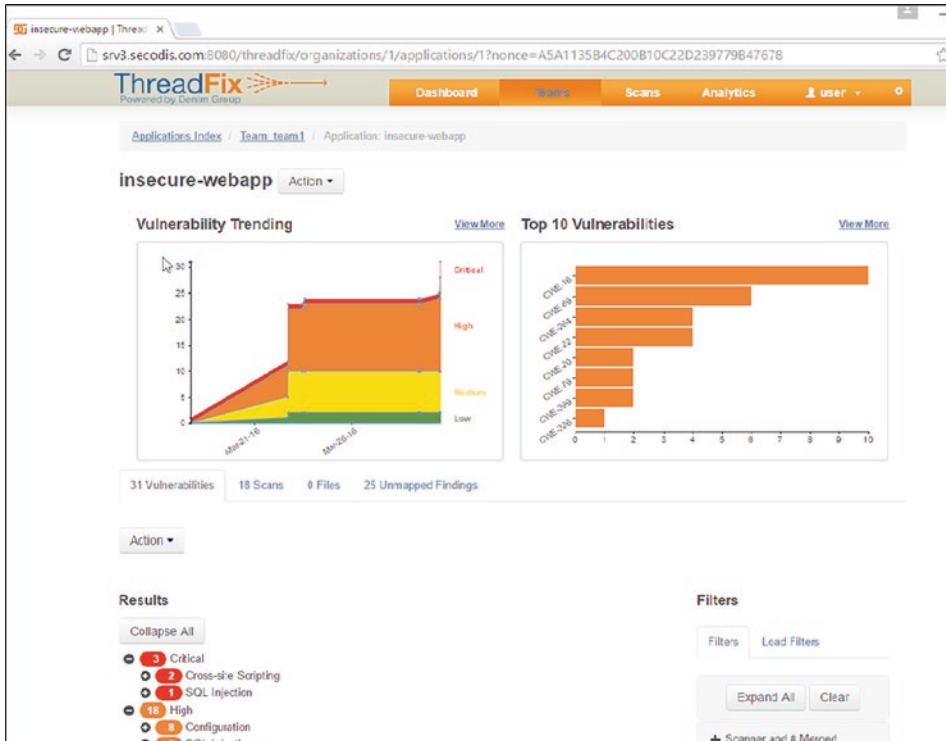
Abb. 4.16 ThreatFix
