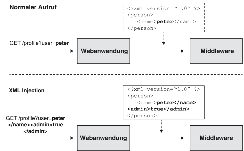
Abb. 2.13 XML Injection
